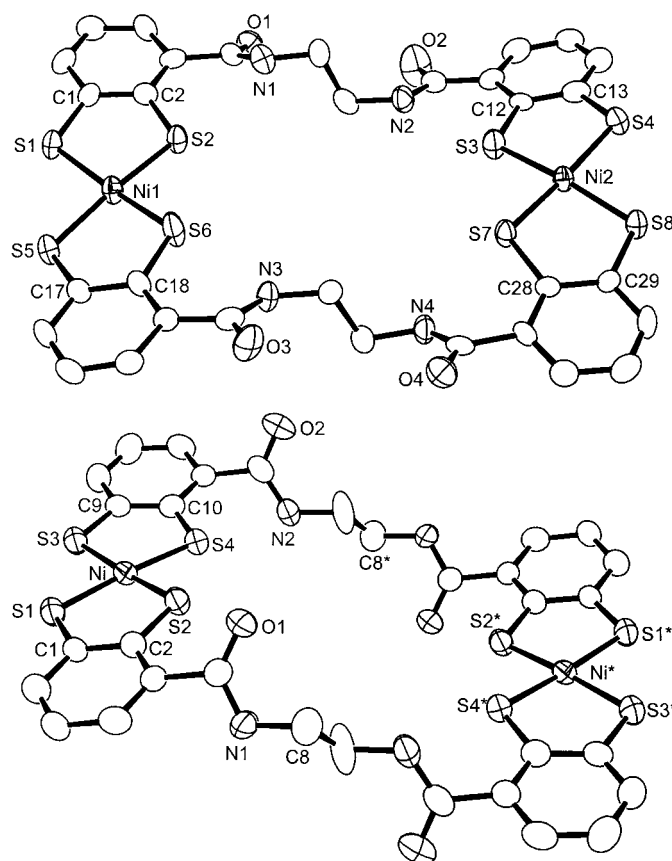
Figure 1. Molecular structures of the nickelate anions in complexes 11b (top) and 13 (bottom) with the crystallographic numbering scheme. Hydrogen atoms, solvent molecules, and cations have been omitted. Starred atoms in the anion of 13 are related to their corresponding atom by a crystallographic inversion center. Selected bond lengths [Å] and angles [°]: 11b Ni1–S1 2.167(2), Ni1–S2 2.161(2), Ni1–S5 2.170(2), Ni1–S6 2.161(2), Ni2–S3 2.162(2), Ni2–S4 2.171(2), Ni2–S7 2.171(2), Ni2–S8 2.167(2), S1–C1 1.768(8), S2–C2 1.743(8), S3–C12 1.767(7), S4–C13 1.766(8), S5–C17 1.742(7), S6–C18 1.753(8), S7–C28 1.765(7), S8–C29 1.749(8); S1–Ni1–S2 91.31(8), S1–Ni1–S5 90.45(8), S1–Ni1–S6 172.34(11), S2–Ni1–S5 174.10(9), S2–Ni1–S6 88.88(8), S5–Ni1–S6 90.13(8), S3–Ni2–S4 89.86(8), S3–Ni2–S7 89.49(8), S3–Ni2–S8 171.44(10), S4–Ni2–S7 174.84(9), S4–Ni2–S8 90.74(8), S7–Ni2–S8 90.67(8), C1–S1–Ni1 105.2(3), C2–S2–Ni1 106.3(3), C12–S3–Ni2 106.8(3), C13–S4–Ni2 105.5(3), C17–S5–Ni1 105.3(3), C18–S6–Ni1 108.4(3), C28–S7–Ni2 106.9(2), C29–S8–Ni2 105.3(3); 13 : Ni–S1 2.140(3), Ni–S2 2.155(3), Ni–S3 2.151(3), Ni–S4 2.162(3), S1–C1 1.730(9), S2–C2 1.742(9), S3–C9 1.736(10), S4–C10 1.756(10), S1–Ni–S2 91.51(10), S1–Ni–S4 175.24(12), S2–Ni–S3 174.84(12), S2–Ni–S4 89.00(10), S3–Ni–S4 91.39(10), C1–S1–Ni 105.1(3), C2–S2–Ni 105.5(3), C9–S3–Ni 105.3(4), C10–S4–Ni 105.4(3).
