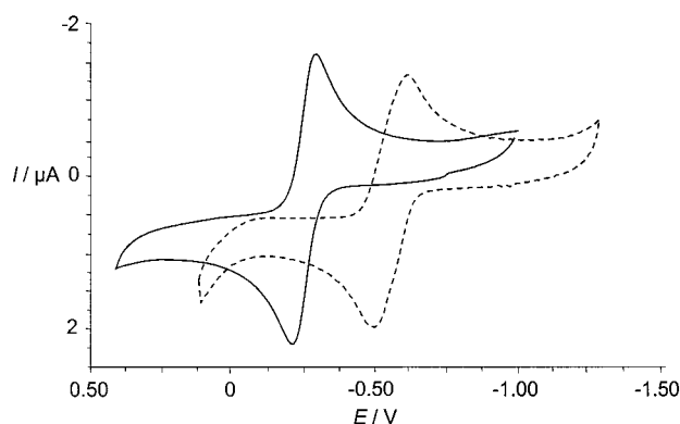
Figure 3. Cyclic voltammograms of 11b (—) and 14 (---) in DMF.
