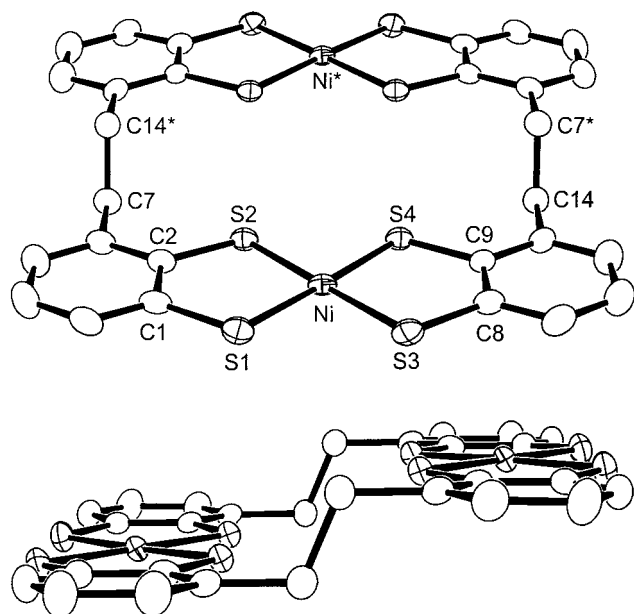
Figure 2. Molecular structure of the nickelate anion in complex 14 (top) and of the stair-type conformation of the nickelate anion (bottom) with the crystallographic numbering scheme. Hydrogen atoms, solvent molecules, and cations have been omitted. Starred atoms are related to their corresponding atom by a crystallographic inversion center. Selected bond lengths [Å] and angles [°]: Ni–S1 2.1712(12), Ni–S2 2.1825(11), Ni–S3 2.1752(12), Ni–S4 2.1727(12), S1–C1 1.766(4), S2–C2 1.756(4), S3–C8 1.768(4), S4–C9 1.757(4); S1–Ni–S2 90.77(4), S1–Ni–S3 90.25(4), S1–Ni–S4 178.03(5), S2–Ni–S3 178.96(5), S2–Ni–S4 87.92(4), S3–Ni–S4 91.06(4), C1–S1–Ni 105.94(14), C2–S2–Ni 105.92(14), C8–S3–Ni 105.41(14), C9–S4–Ni 105.97(14).
