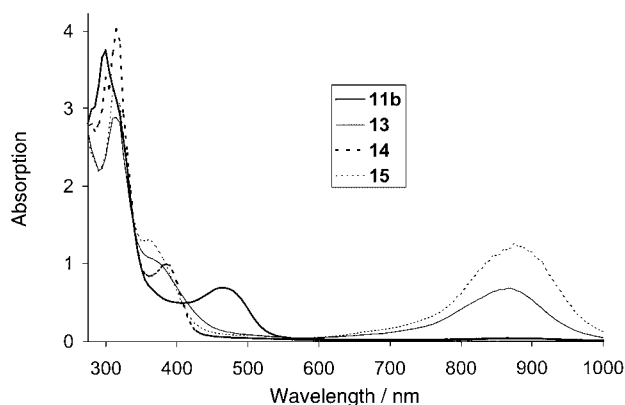
Figure 4. UV/Vis spectra of complexes 11b , 13 , 14 , and 15 in DMF.
