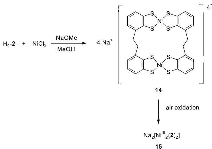
Scheme 4. Preparation of complexes 14 and 15 .
