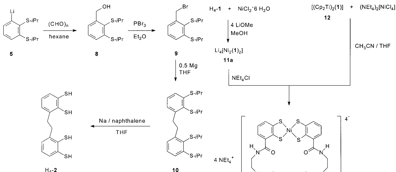
Scheme 2. Synthesis of ligand H_4-2 .
