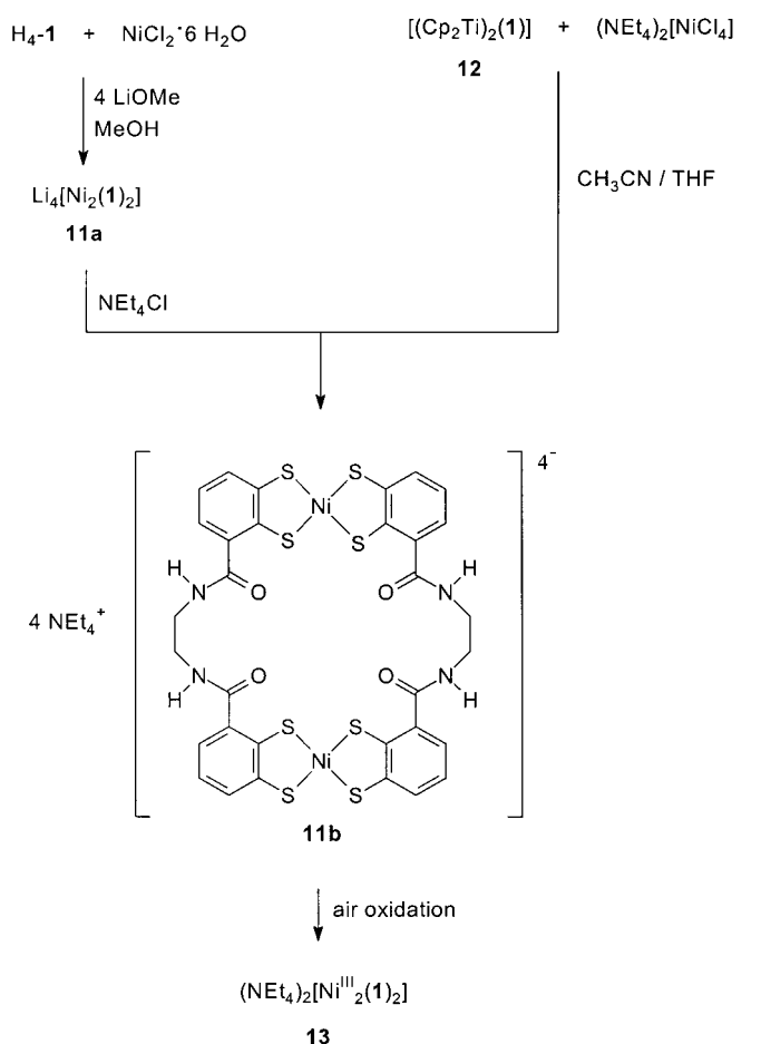
Scheme 3. Preparation of complexes 11a , 11b , and 13 .
