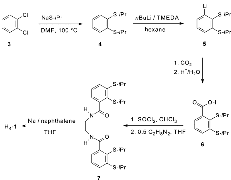
Scheme 1. Synthesis of ligand \text{H}_4\text{-1} .
